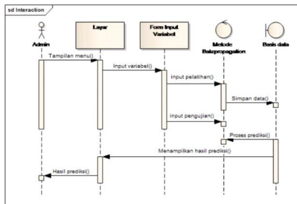
Figure 2. Sequence diagram
