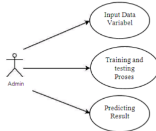
Figure 1. Usecase diagram
