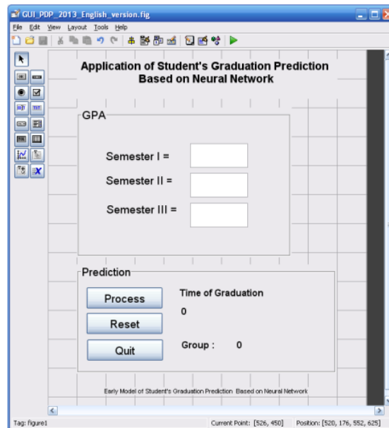
Figure 4. GUI Design
